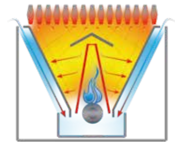
Radiation heating system. Patented (US9591947B2 and related family)
